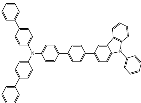
Compound B
