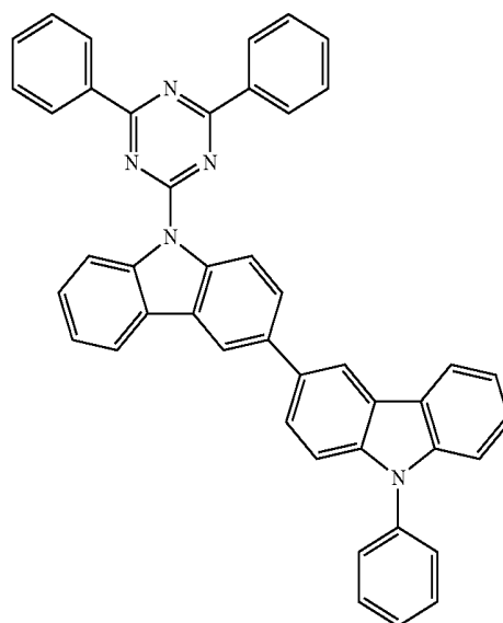
Compound 5
