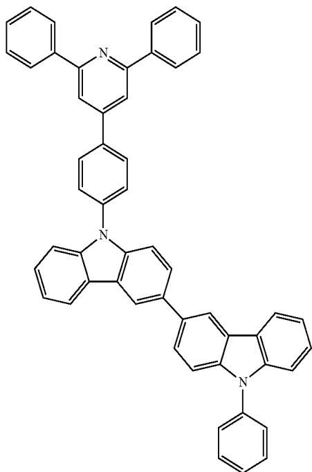
Compound 2
