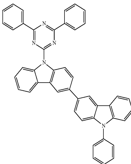
Compound 5
