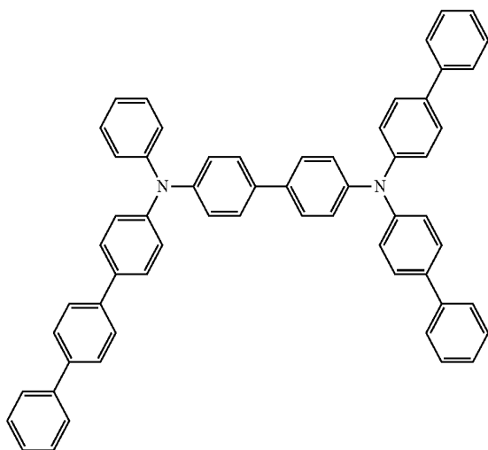
Compound A
