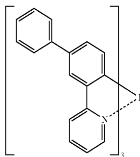
Ir(Ph-ppy) 3 (facial body)
