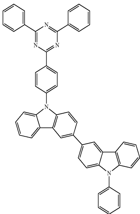
Compound 3
