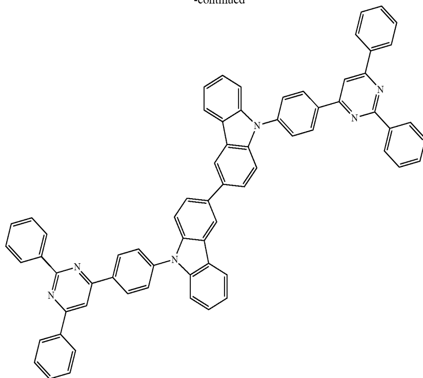
Compound 4
