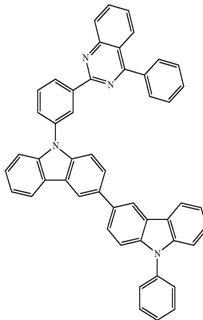
Compound 8
