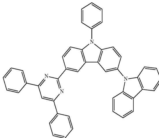
Compound G
