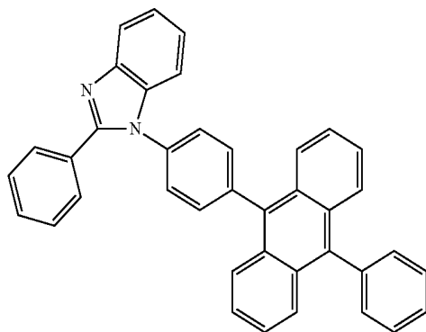
Compound C
