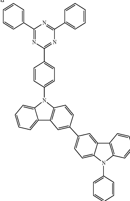
Compound 3
